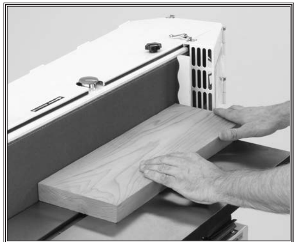
Figure 31. Edge sanding with the Model W1730.
