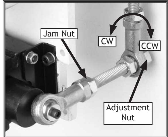
Figure 22. Jam and adjustment nuts, clockwise (CW) and Counter Clockwise (CCW) rotation.
