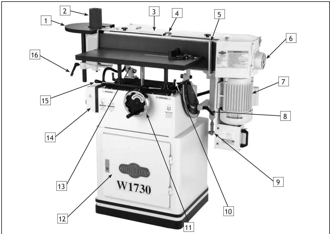
Figure 1. Controls and Features of the W1730.
