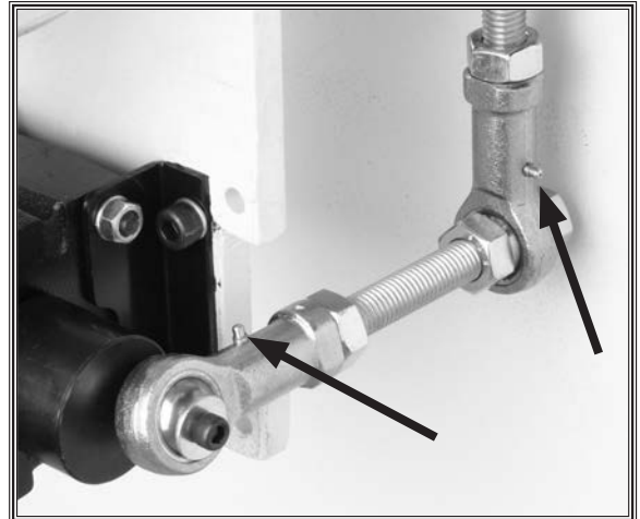
Figure 33. Oil ports.
