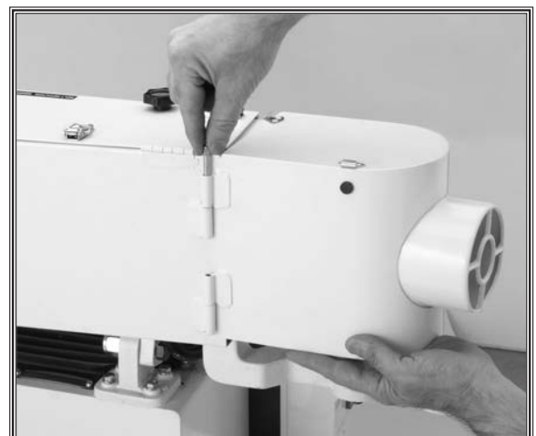
Figure 16. Inserting dust port cover hinge pin.
