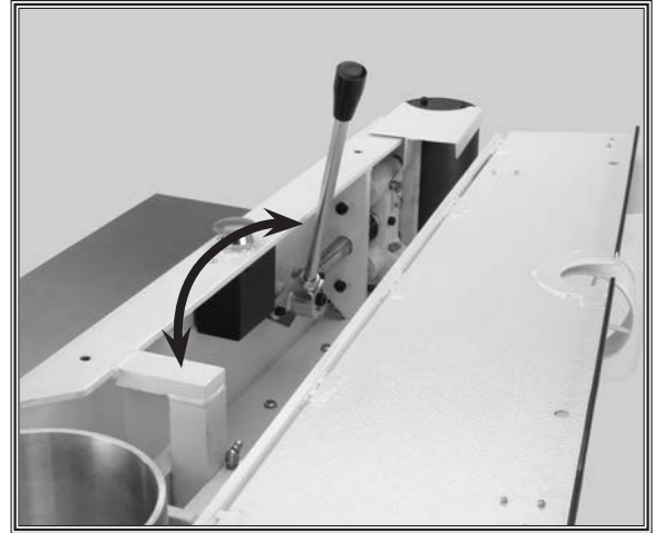
Figure 11. Released position of the belt tensioning lever.
