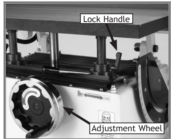
Figure 25. Vertical table adjustment.
