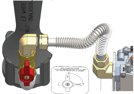
FIG. 15 Natural Gas position, Premier 170 shown
