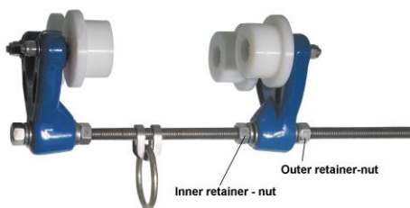
Fig. 3.7 FallTech Beam Trolley (7710)
