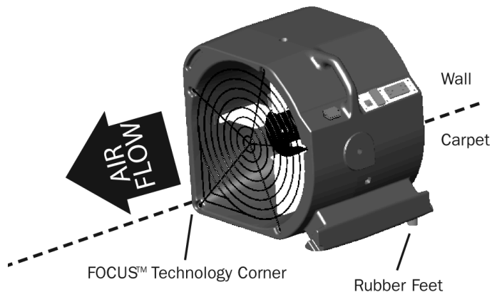
Figure 6: Placement for counter-clockwise drying
