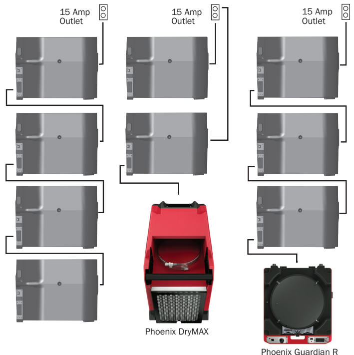
Figure 2: Duplex GFCI use
