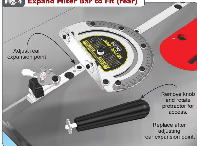
Fig. 4 Expand Miter Bar to Fit (rear)
