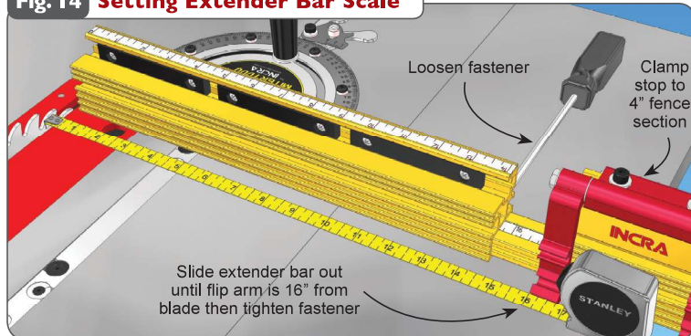
Fig. 14 Setting Extender Bar Scale
