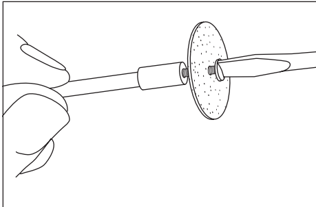
Mandrel No. 402 has a small screw at its tip, and is used with emery cutting wheels and sanding discs.
