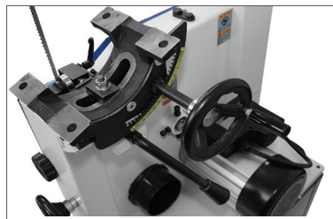
QUICK-LOCK CAST IRON TRUNNION SYSTEM
