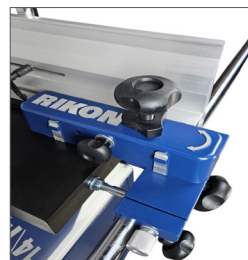
NEW DRIFTX 6" TALL RIP FENCE SYSTEM WITH MICRO-ADJUSTMENT
