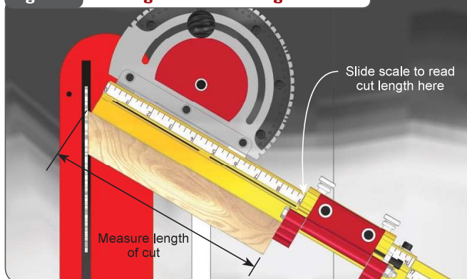
Fig. 15 Micro Adjusting
