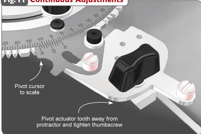
Fig. 11 Continuous Adjustments
