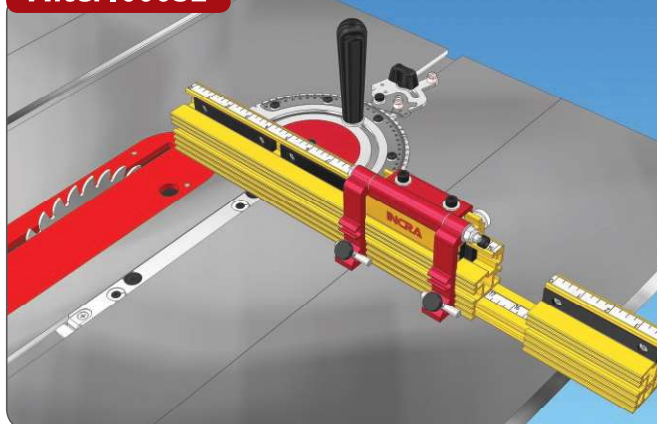
Fig. 9 Changing Angles
