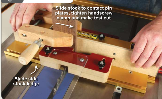
Fig. 20 Make Test Cut
