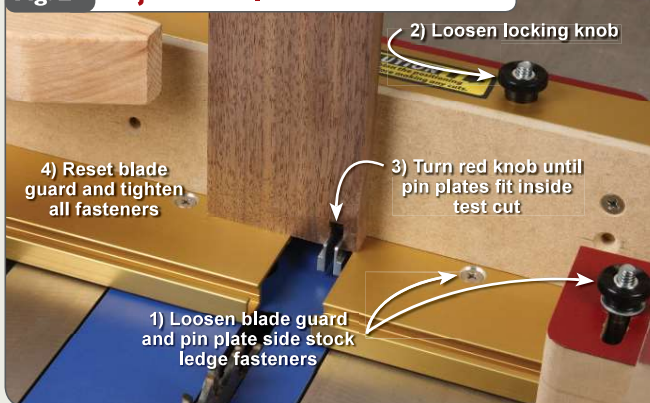
Fig. 21 Adjust Pin Plates to Fit Test Cut
