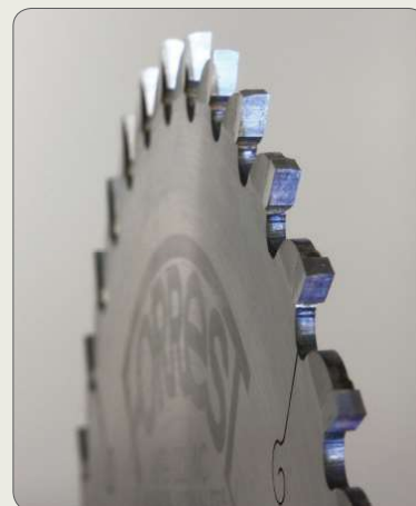
Special Grind Box Joint Blade
