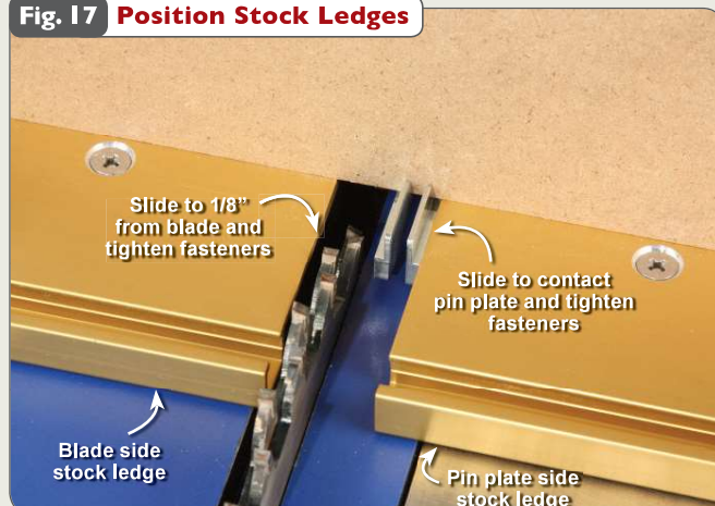
Fig. 17 Position Stock Ledges
