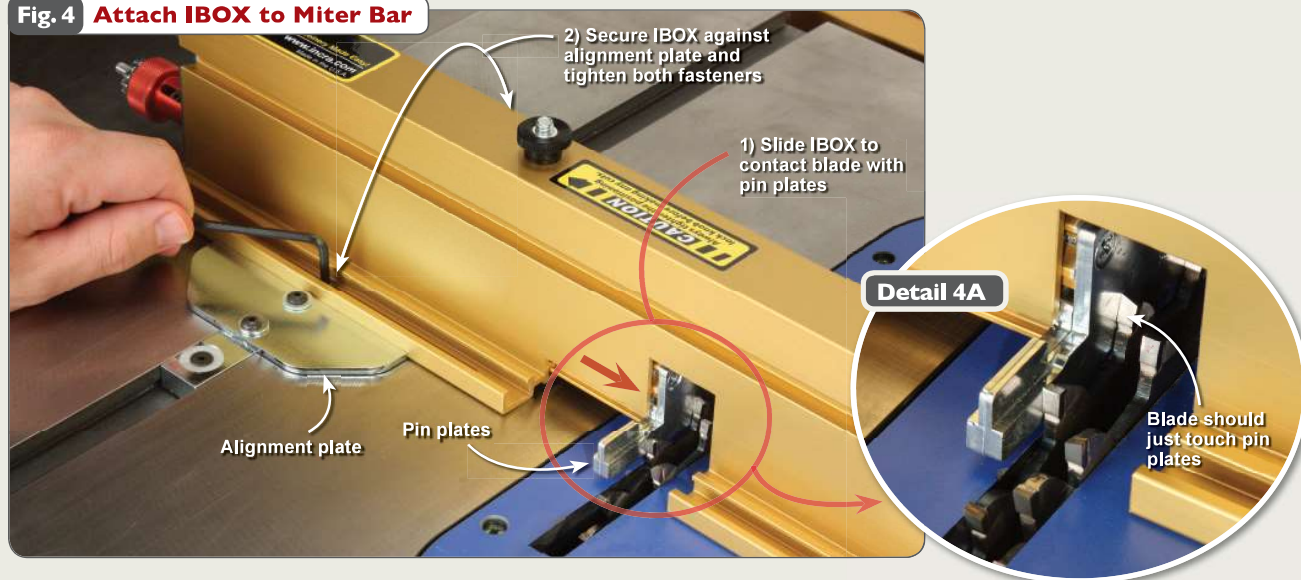
Fig. 4 Attach IBOX to Miter Bar
