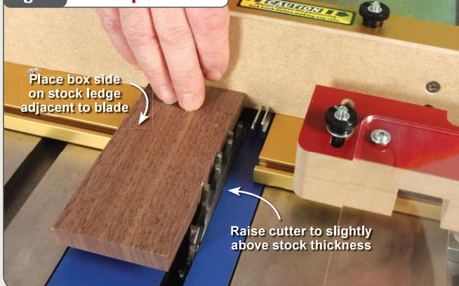
Fig. 18 Set Depth of Cut
