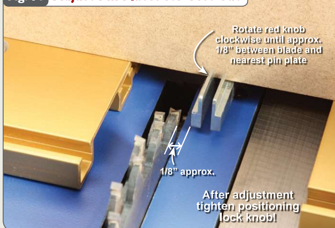
Fig. 16 Adjust Pin Plates for Test Cut
