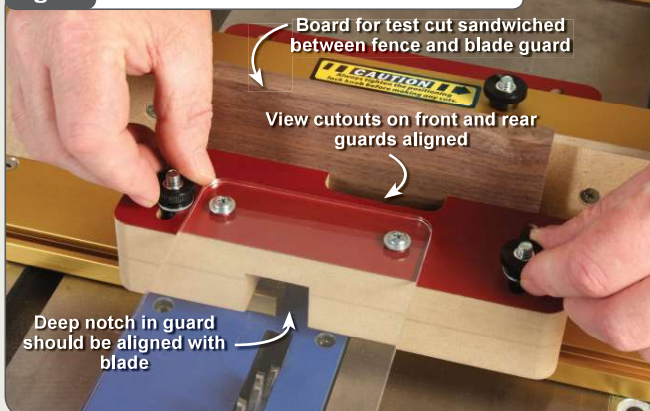
Fig. 19 Position and Secure Blade Guard
